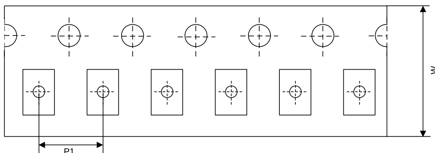
Tape Dimensions
