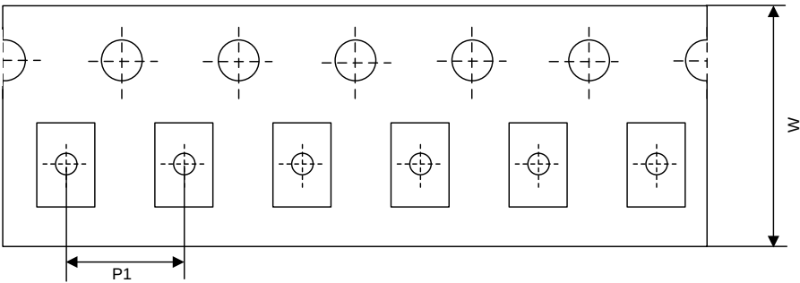
Tape Dimensions
