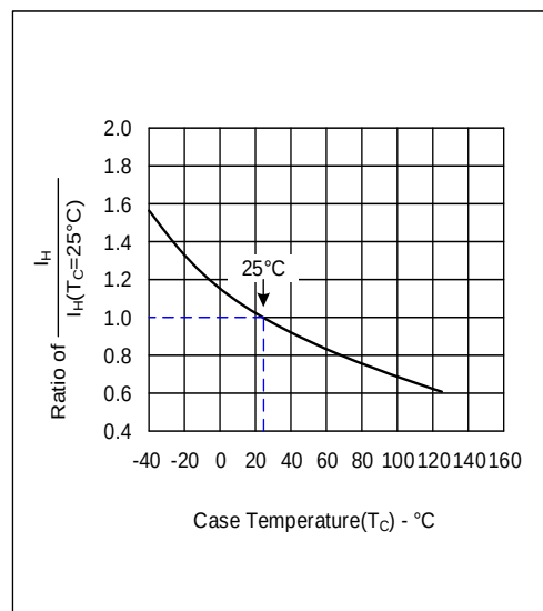
Normalized DC Holding Current versus Case Temperature
