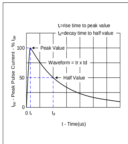
t_r \times t_d Pulse Waveform
