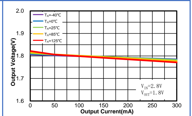
Figure 2. WR0332-18A50R-AT Load Regulation vs. I_{OUT} & Ambient Temperature
