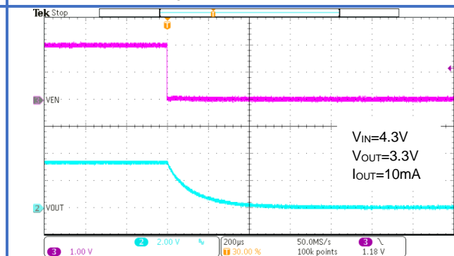
Figure 31. EN Shutdown
