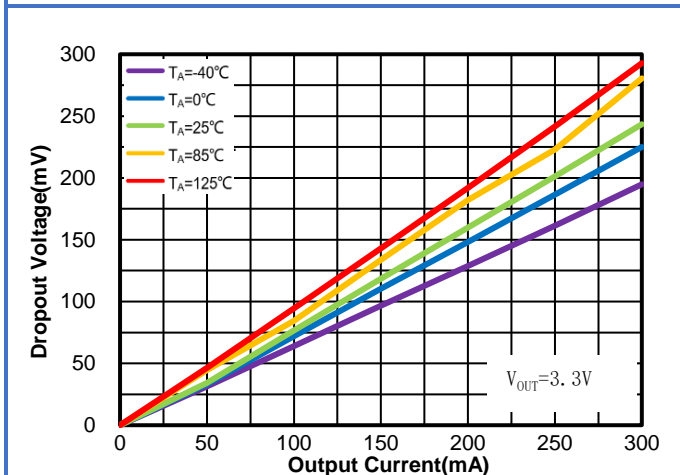
Figure 3. WR0332-33A50R-AT Dropout Voltage vs. I_{OUT} & Ambient Temperature
