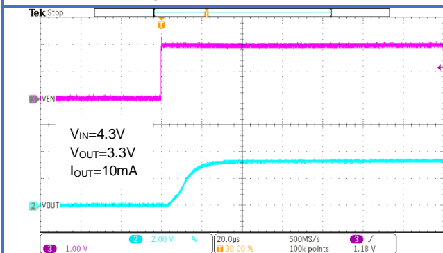
Figure 30. Soft Start from EN
