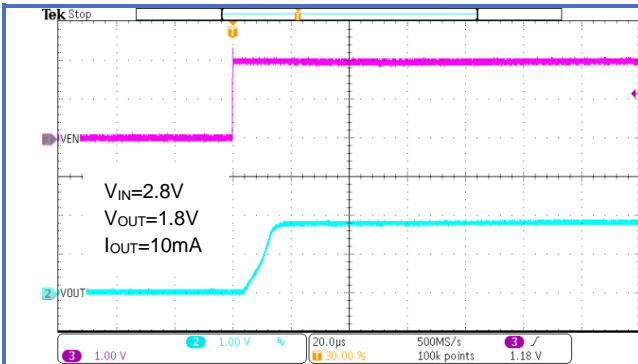
Figure 28. Soft Start from EN
