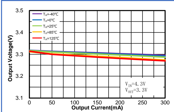
Figure 1. WR0332-33A50R-AT Load Regulation vs. I_{OUT} & Ambient Temperature
