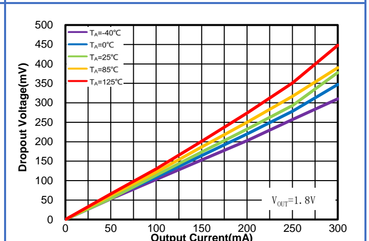
Figure 4. WR0332-18A50R-AT Dropout Voltage vs. I_{OUT} & Ambient Temperature
