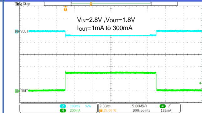
Figure 33. Load Transient
