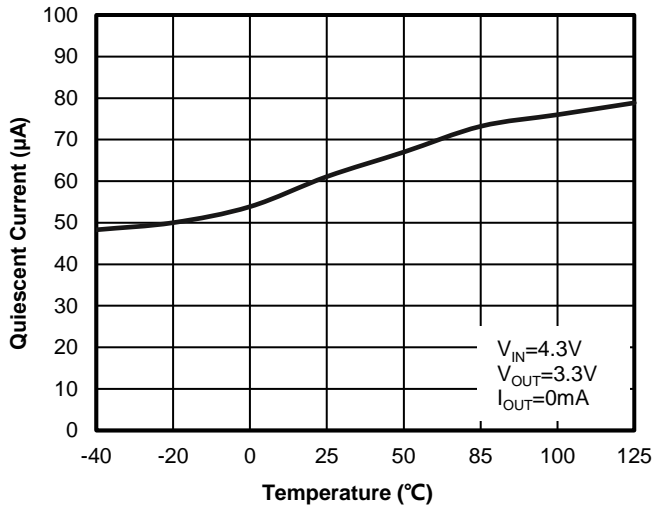
Figure 25. WR0332-33A50R-AT Quiescent Current vs. Ambient Temperature
