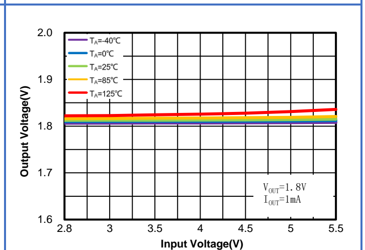
Figure 6. WR0332-18A50R-AT Regulation vs. V_{IN} (Line Regulation) & Ambient Temperature
