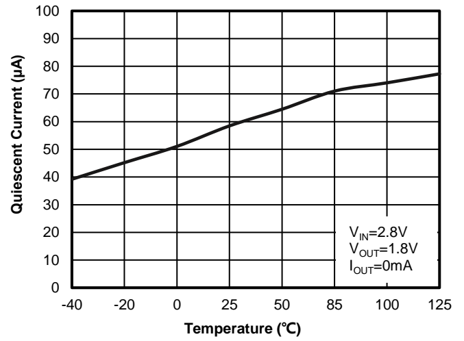
Figure 26. WR0332-18A50R-AT Quiescent Current vs. Ambient Temperature
