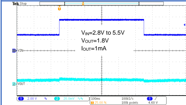
Figure 32. Line Transient
