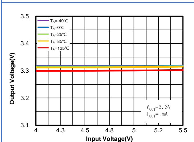
Figure 5. WR0332-33A50R-AT Regulation vs. V_{IN} (Line Regulation) & Ambient Temperature
