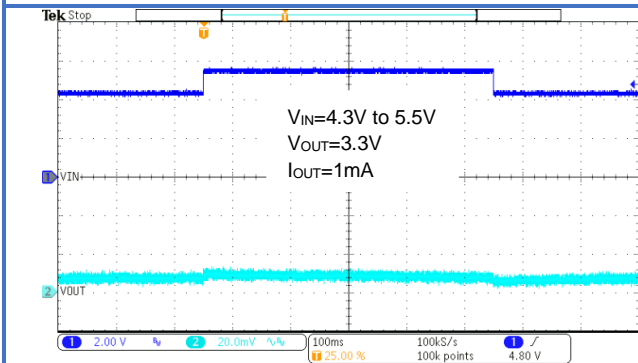
Figure 34. Line Transient
