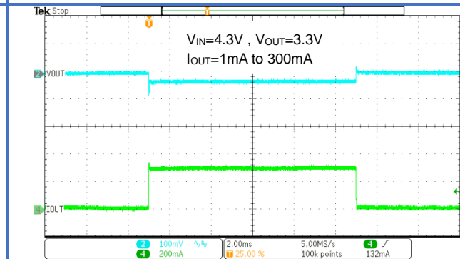
Figure 35. Load Transient
