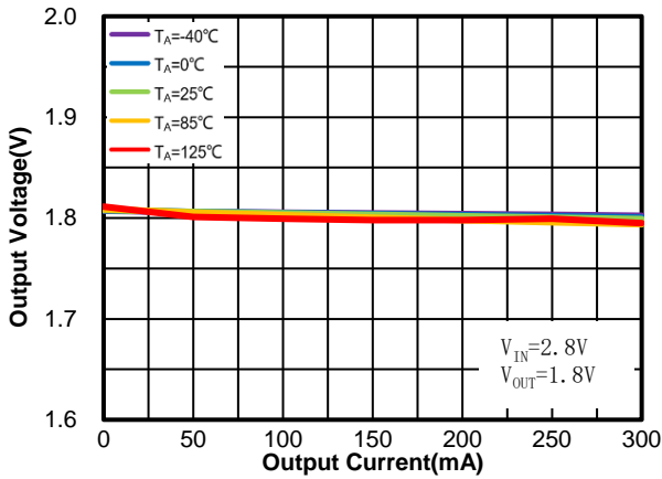
Figure 1. WR0332-18FF4R
