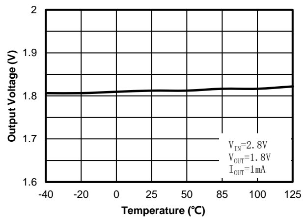
Figure 46. WR0332-18A50R
