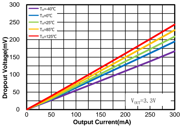
Figure 7. WR0332-33FF4R
