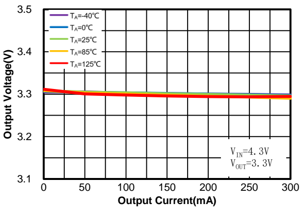
Figure 3. WR0332-33FF4R
