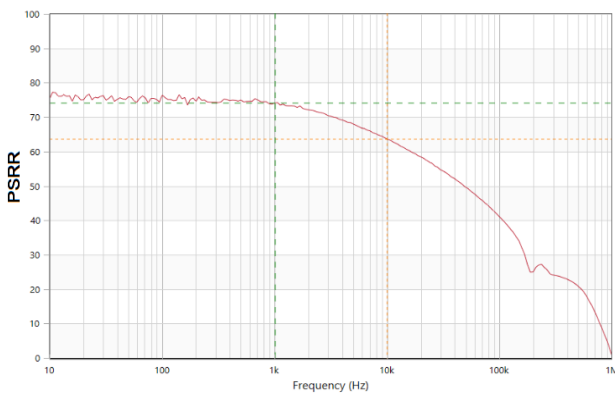
Figure 53. Power Supply Rejection Ratio vs. Frequency
