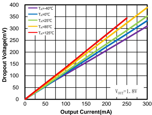
Figure 5. WR0332-18FF4R
