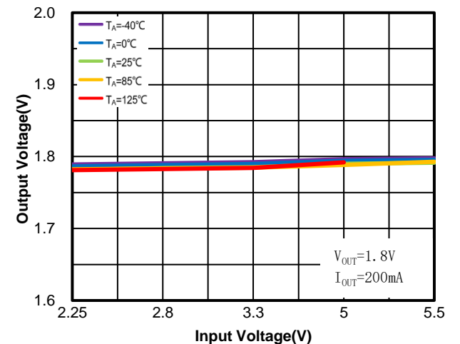
Figure18. WR0332-18A50R
