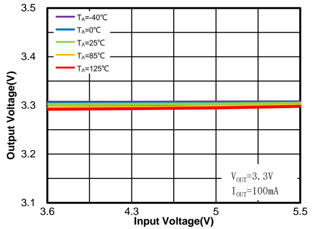
Figure 16. WR0332-33A50R
