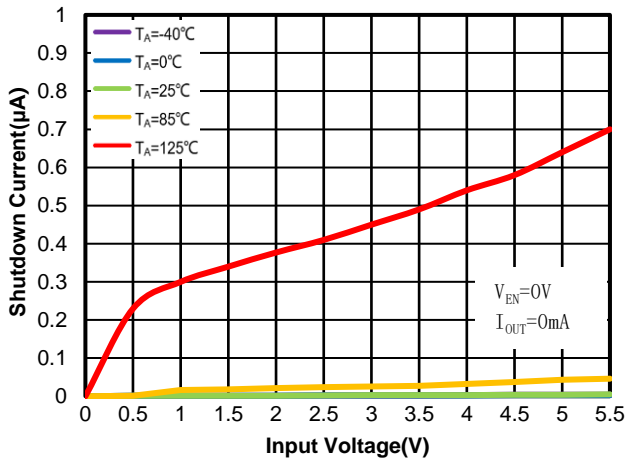
Figure 33. WR0332-18FF4R
