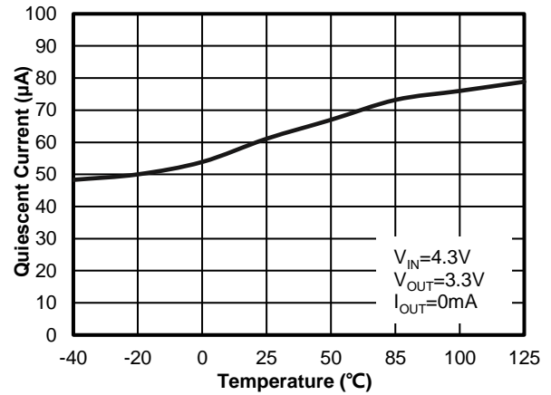
Figure 52. WR0332-33A50R
