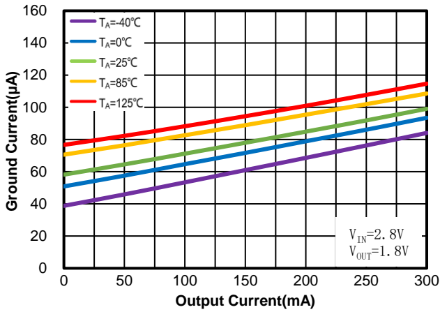
Figure 25. WR0332-18FF4R
