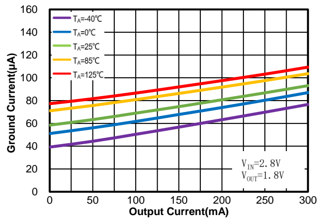
Figure 26. WR0332-18A50R
