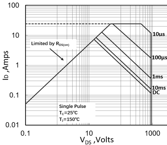
Figure 9. Maximum Safe Operating Area (TO-220/TO-263)
