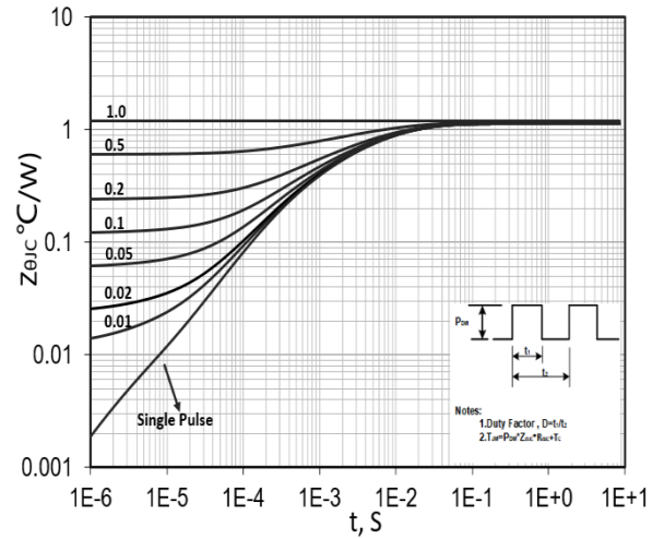
Figure 10. Transient Thermal Response Curve (TO-220/TO-263)
