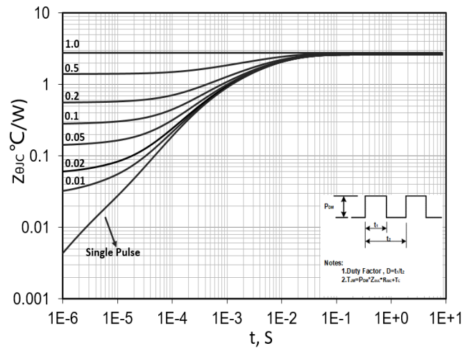
Figure 10. Transient Thermal Response Curve (TO-252)
