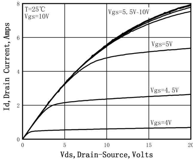
Figure 1. On-Region Characteristics
