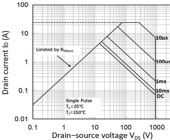
Figure 9. Maximum Safe Operating Area (TO-220/TO-263)
