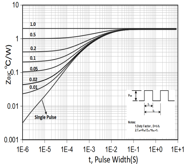
Figure 10. Transient Thermal Response Curve (TO-220/TO-263)
