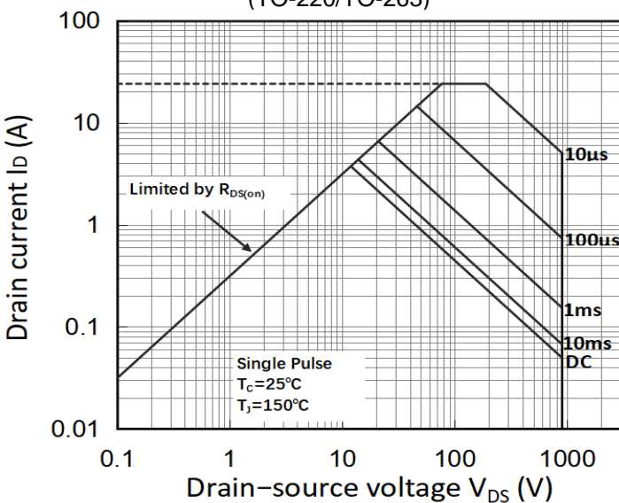
Figure 11. Maximum Safe Operating Area (TO-220F)
