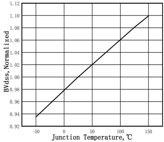
Figure 6. Normalized BV_{DSS} vs. Temperature
