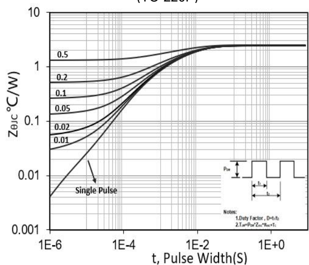
Figure 12. Transient Thermal Response Curve (TO-252/TO-251-L4.0)
