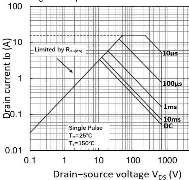
Figure 9. Maximum Safe Operating Area (TO-220F)
