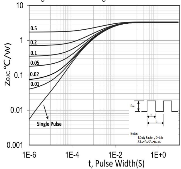
Figure 10. Transient Thermal Response Curve (TO-220F)
