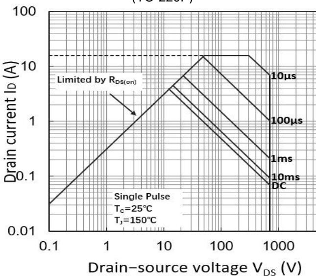
Figure 11. Maximum Safe Operating Area (TO-252/TO-251-L4.0)
