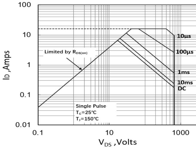
Figure 13. Maximum Safe Operating Area (TO-252)
