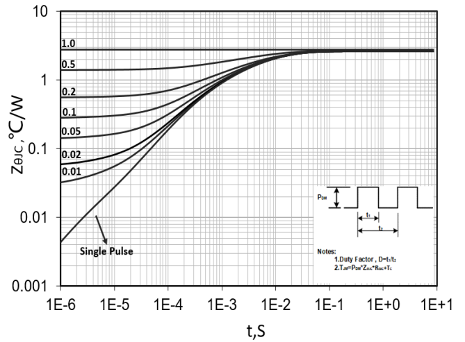
Figure 10. Transient Thermal Response Curve (TO-220F)
