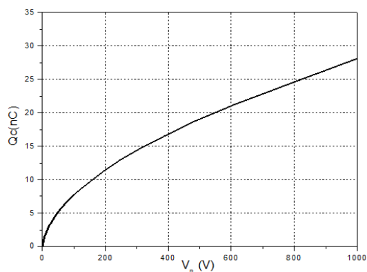
Fig.3-Total Capacitance Charge VS Reverse Voltage
