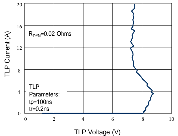
Figure 6: TLP Curve
