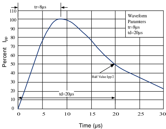
Figure 5: Pulse Waveform
