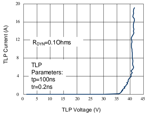
Figure 6: TLP Curve
