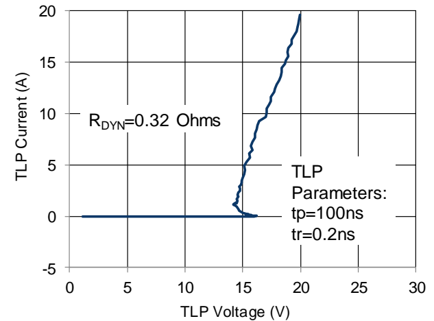
Figure 6: TLP Curve
