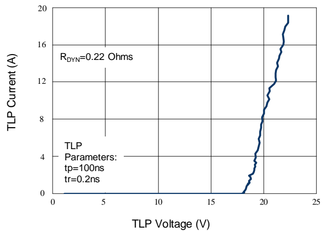
Figure 6: TLP Curve
