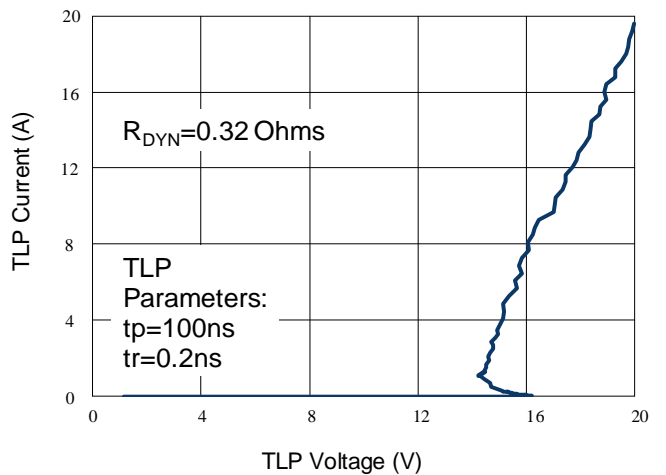
Figure 6: TLP Curve
