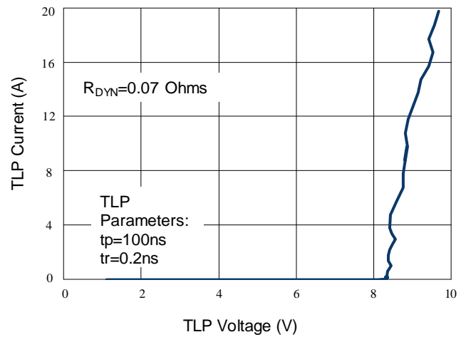
Figure 6: TLP Curve
