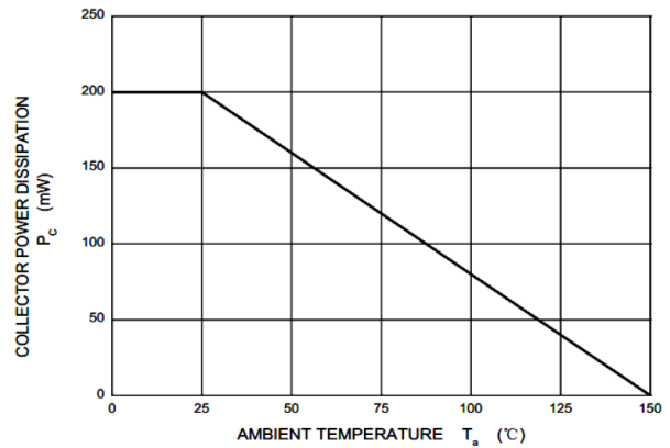
Figure 8. P_c vs. T_a
