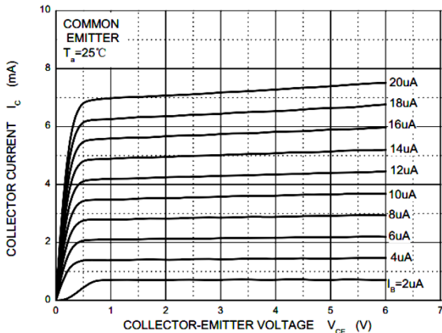
Figure 1. Static Characteristics
