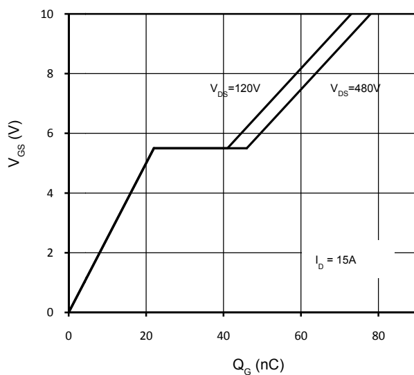
Figure 15. Gate Charge Characteristics
