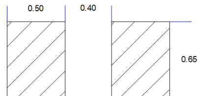
Recommended soldering dimension
