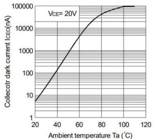
Fig.6 Collector Dark Current vs Ambient Temperature
