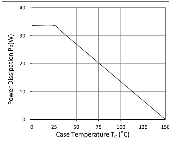
Figure 9. Power Dissipation
