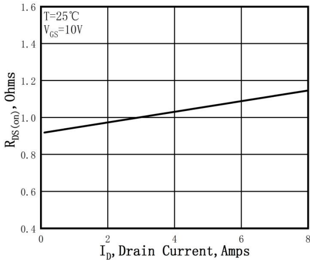
Figure 3. Static Drain-Source On Resistance
