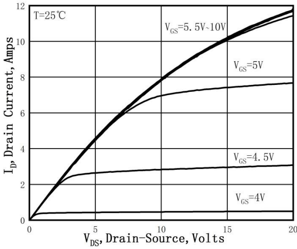
Figure 1. On-Region Characteristics
