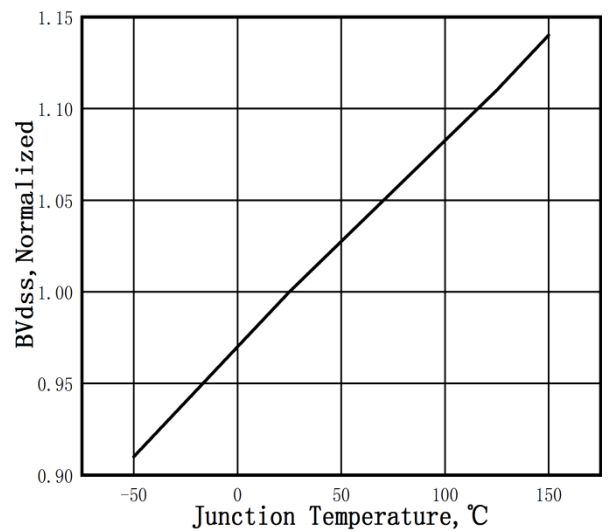
Figure 6. Normalized BV_{DS} vs. Temperature
