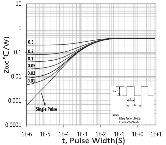
Figure 10. Transient Thermal Response Curve
