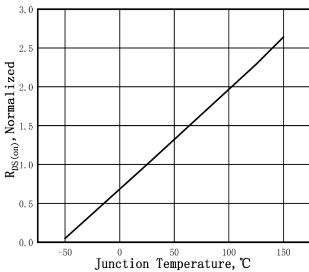
Figure 5. Normalized R_{DS(on)} vs. Temperature
