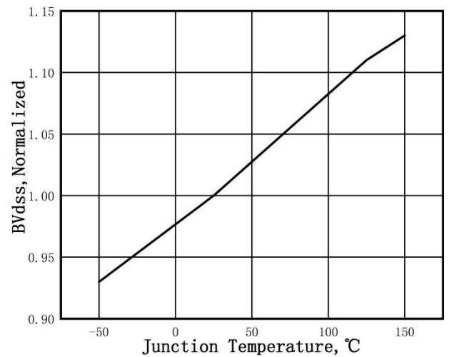
Figure 6. Normalized BV_{DS} vs. Temperature
