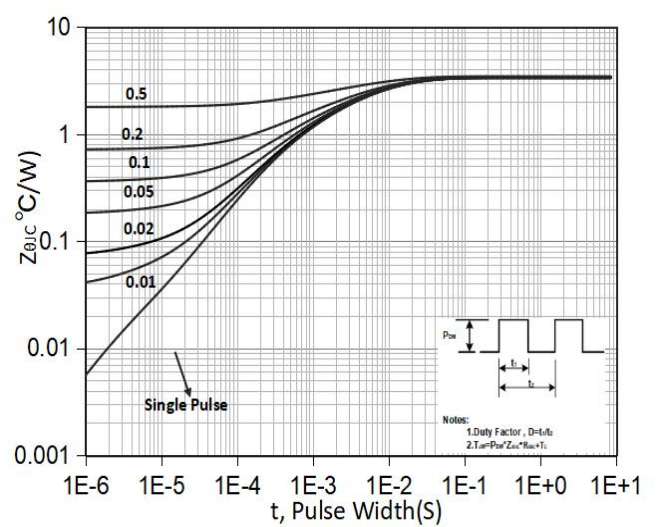
Figure 10. Transient Thermal Response Curve (TO-247-3L)
