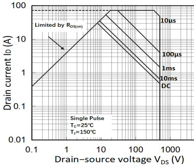
Figure 13. Maximum Safe Operating Area (TO-220)
