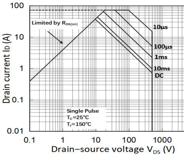
Figure 9. Maximum Safe Operating Area (TO-247-3L)
