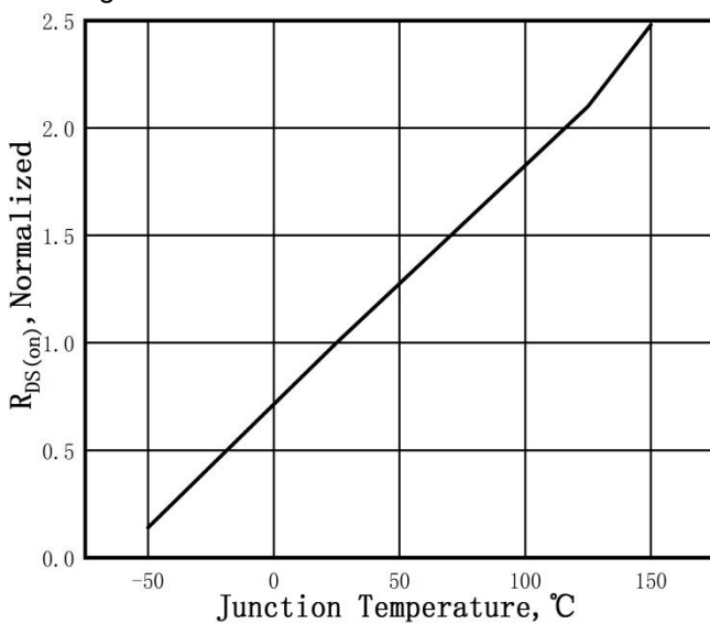
Figure 5. Normalized R_{DS(on)} vs. Temperature
