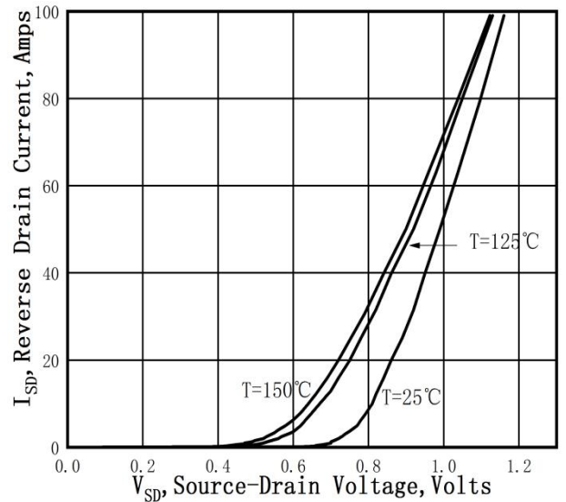
Figure 4. Typical Body Diode Transfer Characteristics
