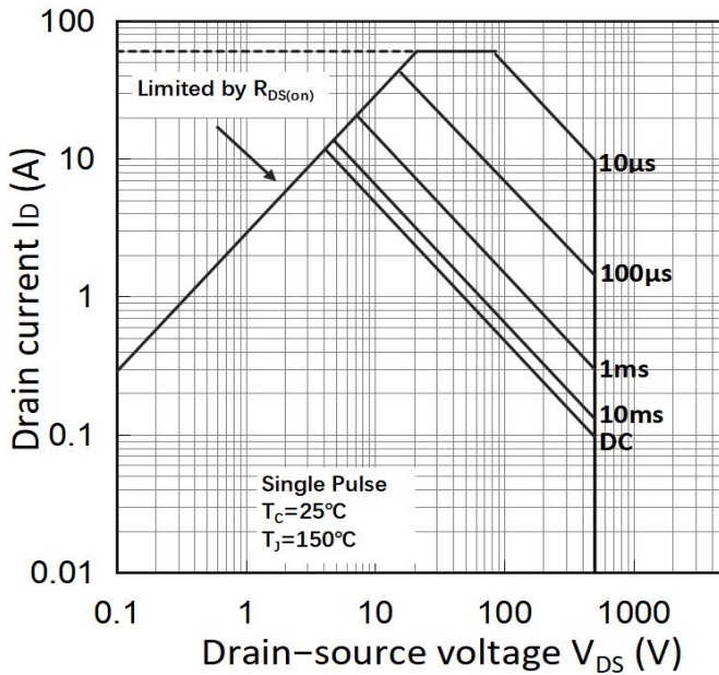
Figure 9. Maximum Safe Operating Area (TO-220F)
