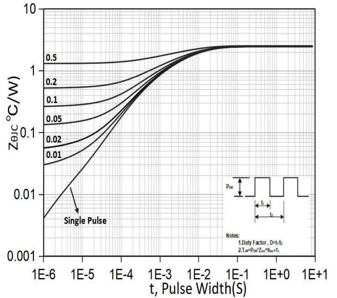
Figure 10. Transient Thermal Response Curve (TO-220F)
