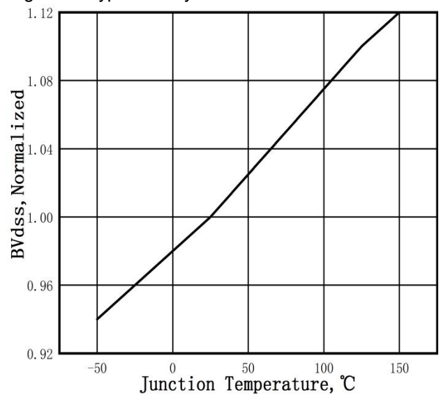
Figure 6. Normalized BV_{DSS} vs. Temperature
