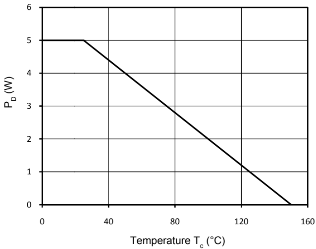
Figure 9. Power Dissipation
