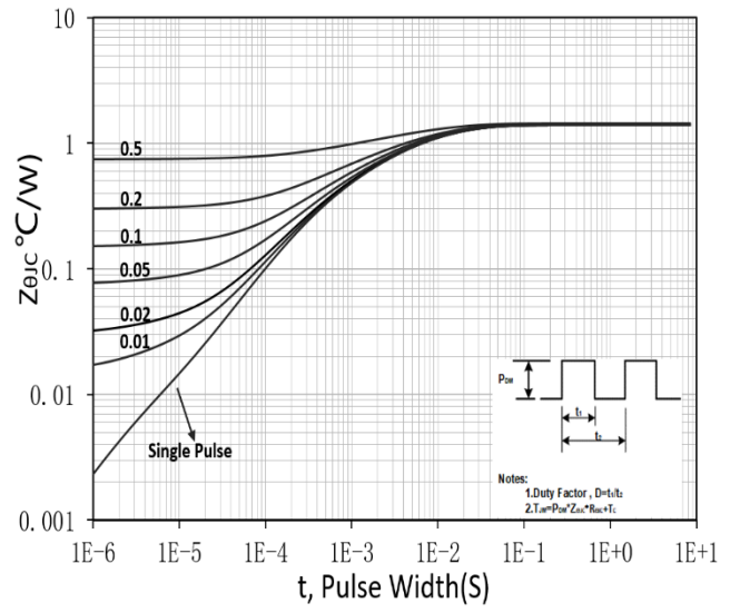
Figure 14. Transient Thermal Response Curve (TO-252)
