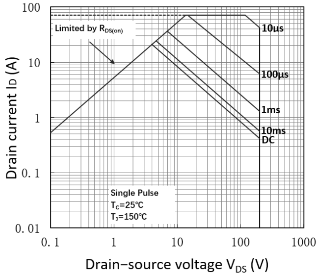
Figure 13. Maximum Safe Operating Area (TO-252)
