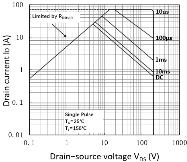
Figure 9. Maximum Safe Operating Area (TO-220)
