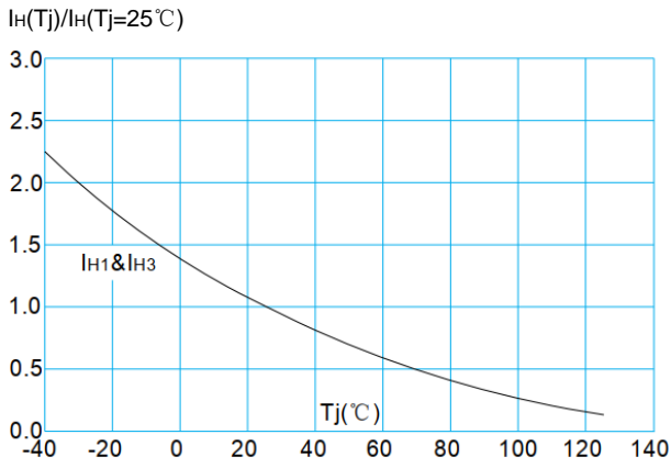
FIG. 7: Relative variations of holding current versus junction temperature FIG. 8: Relative variations of latching current versus junction temperature
