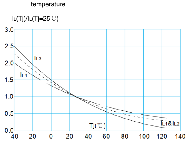
FIG. 7: Relative variations of holding current versus junction temperature FIG. 8: Relative variations of latching current versus junction temperature
