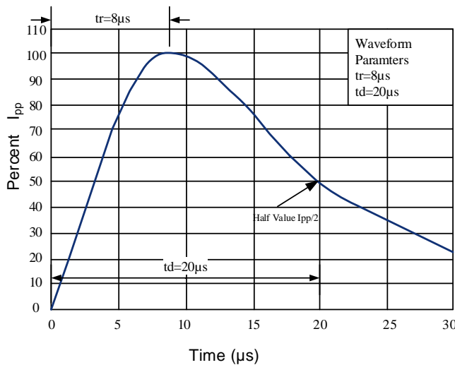
Figure 5: 8/20μs Pulse Waveform
