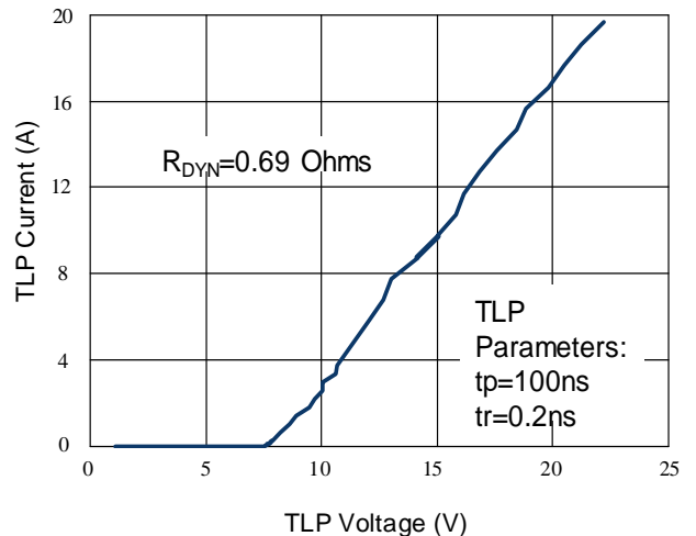
Figure 6: TLP Curve
