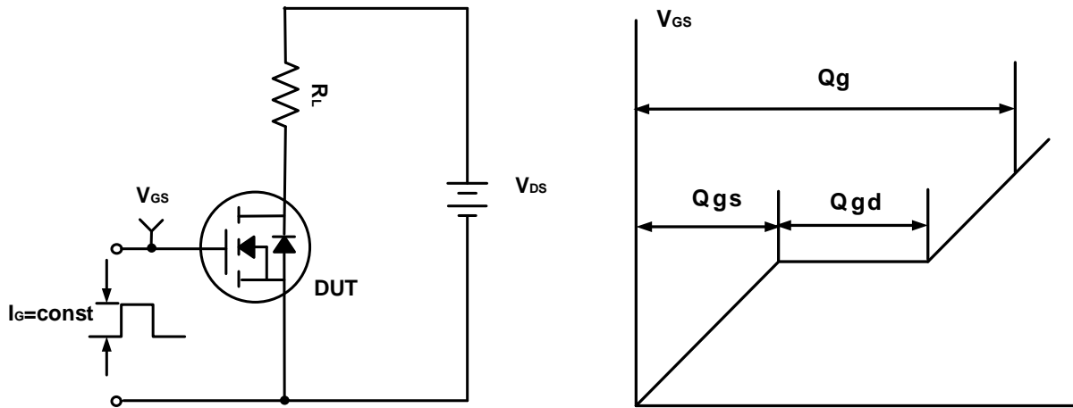
Figure A. Gate Charge Test Circuit & Waveforms
