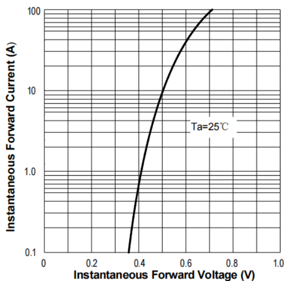
FIG.3: Forward Voltage
