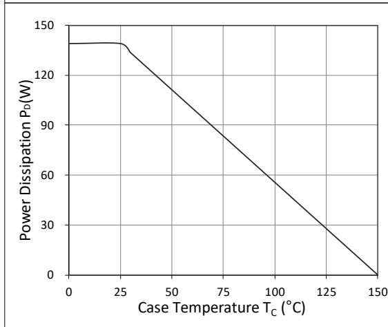
Figure 9. Power Dissipation
