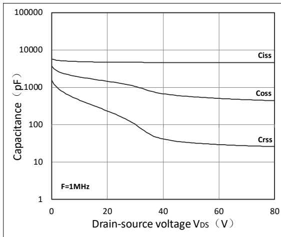
Figure 7. Capacitance Characteristics
