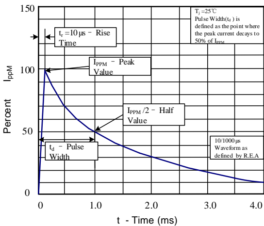
Figure 3: Pulse Waveform
