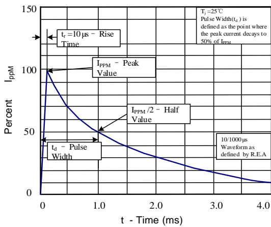
Figure 3: Pulse Waveform
