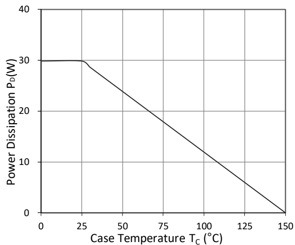
Figure 9. Power Dissipation
