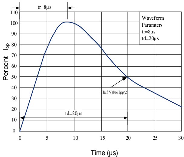
Figure 5: Pulse Waveform
