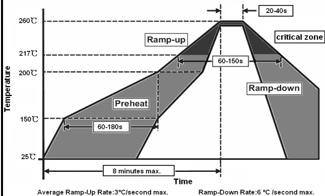
Average Ramp-Up Rate: 3°C/second max. Ramp-Down Rate: 5°C/second max.
